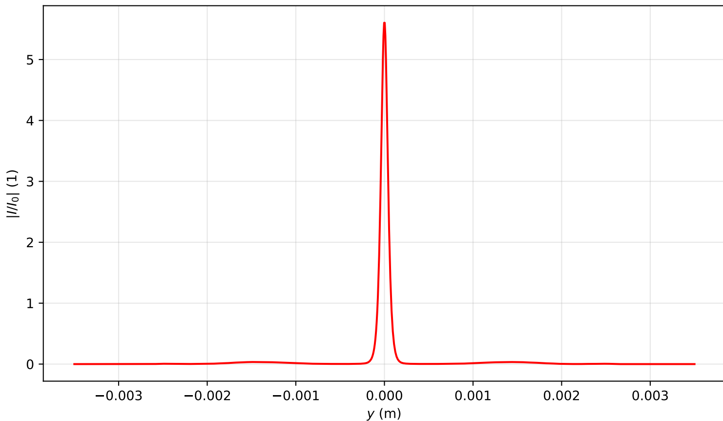
Intensity profile I(x=0, y, z=1.115)/I_0 , P_{in}=7.0P_{cr} , artificial time
